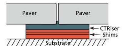
Fig.3 Multiple shims of the same or different thicknesses can be combined to make up the exact height required.
