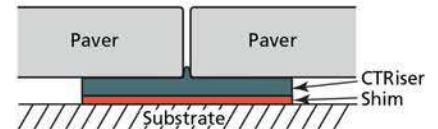
Fig.2 Shims of the appropriate thickness can be used individually or combined to level the pavers over uneven surfaces up to 6" in height.
